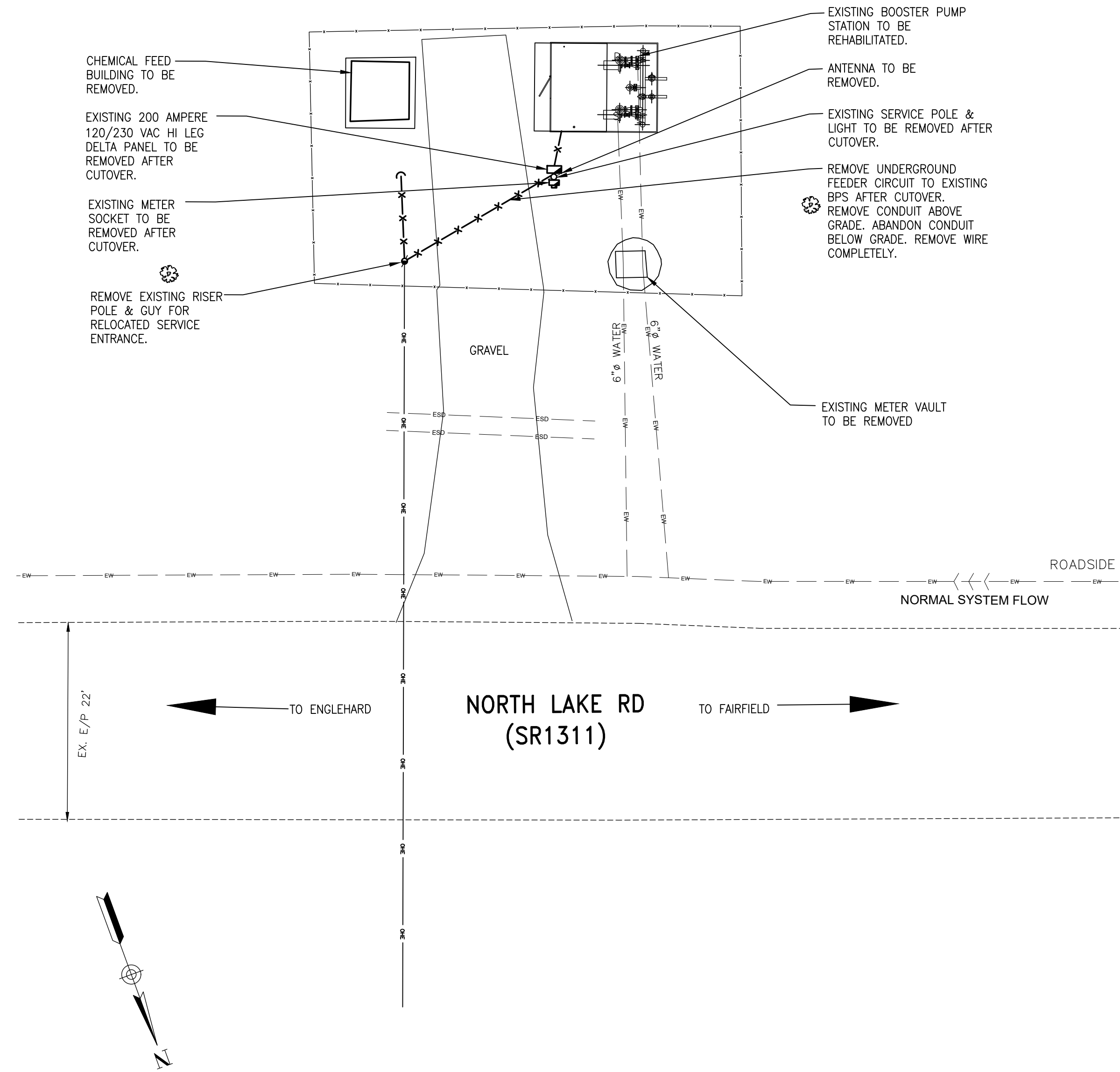
1 DANIELS ELECTRICAL SITE PLAN E-7 DEMOLITION 1"=10'-0"
