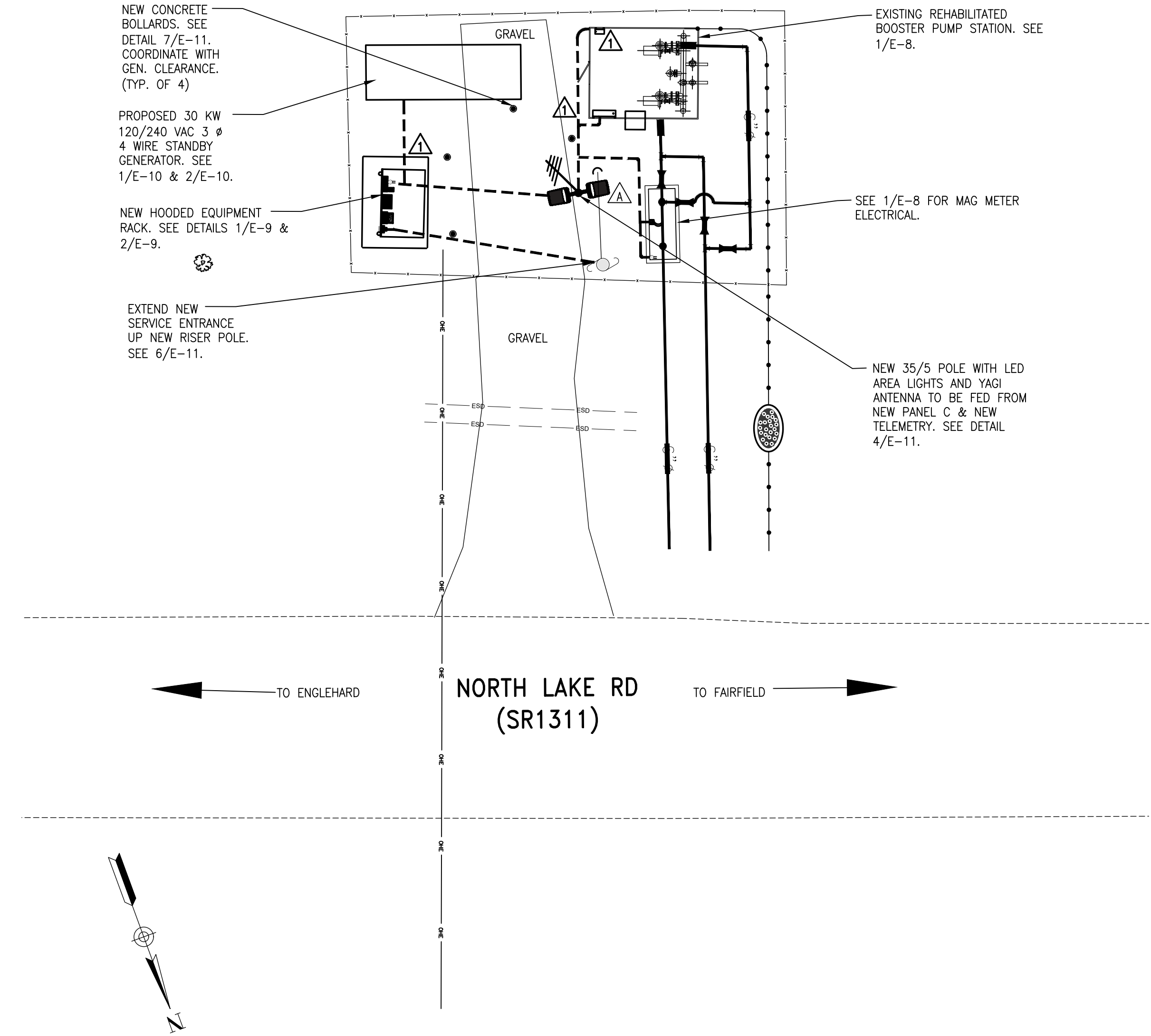
2 DANIELS ELECTRICAL SITE PLAN E-7 INSTALLATION 1"=10'-0"
